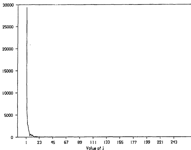
FIGURE 6.4 Sample periodogram for the data plotted in Figure 6.3. The figure plots \hat{f}_y(\omega_j) as a function of j , where \omega_j = 2\pi j/T .
