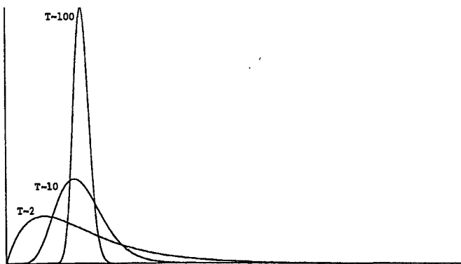
FIGURE 7.1 Density of the sample mean for a sample of size T .
