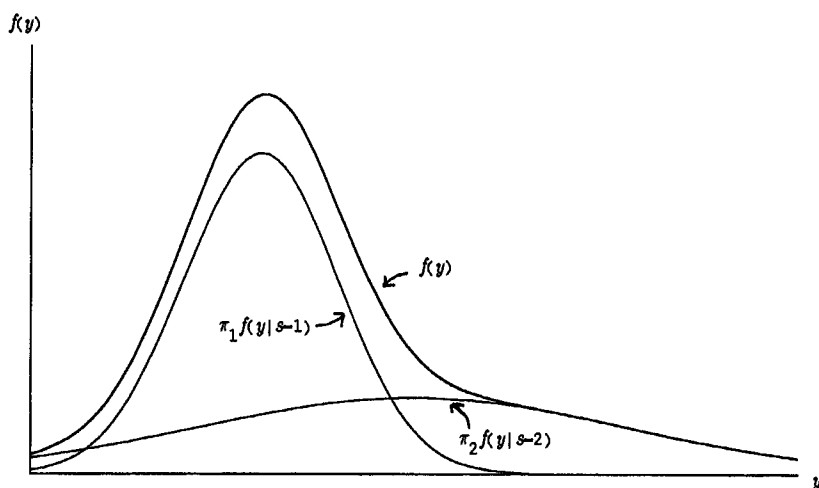
FIGURE 22.3 Density of mixture of two Gaussian distributions with y_i|s_i = 1 \sim N(0, 1) , y_i|s_i = 2 \sim N(2, 8) , and P\{s_i = 1\} = 0.6 .
