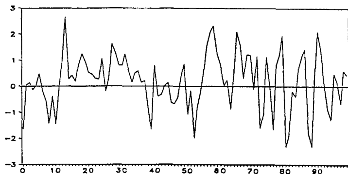
(b) \phi = 0.5
