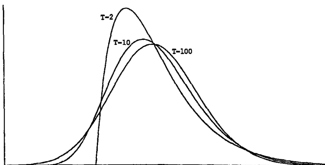
FIGURE 7.2 Density of \sqrt{T}(\bar{Y}_T - \mu) .
