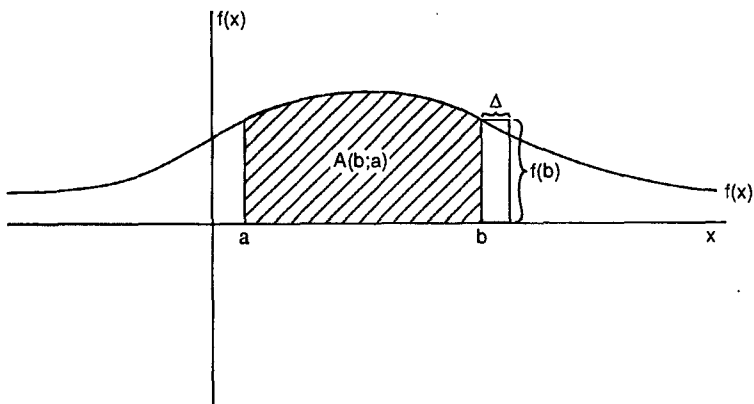
FIGURE A.5 The definite integral as the area under a function.
