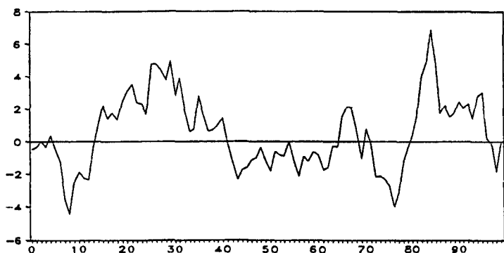
(c) \phi = 0.9
