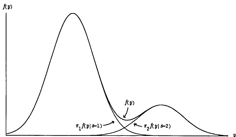
FIGURE 22.2 Density of mixture of two Gaussian distributions with y_i|s_i = 1 \sim N(0, 1) , y_i|s_i = 2 \sim N(4, 1) , and P\{s_i = 1\} = 0.8 .
