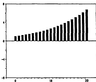
(c) \phi = 1.1
