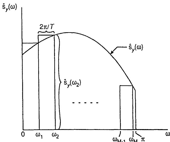
FIGURE 6.2 The area under the sample periodogram and the portion of the variance of y attributable to cycles of different frequencies.
