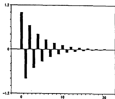
(b) \phi = -0.8
