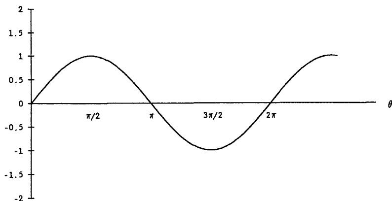
(a) \sin(\theta)
