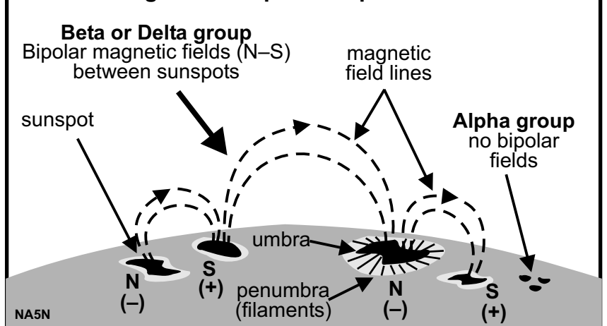
Fig. 3 – Sunspot Groups Illustrated
