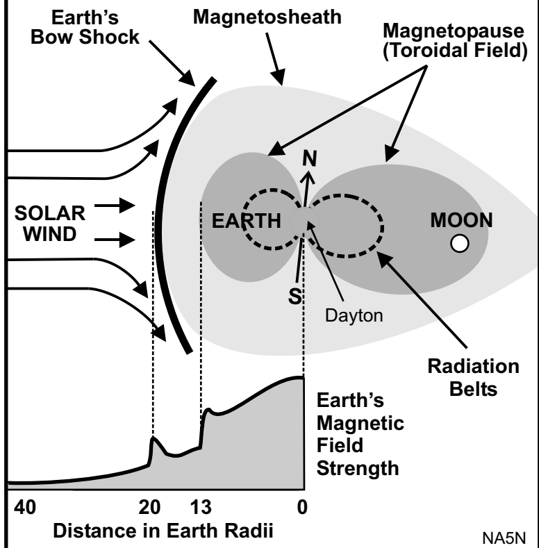
Fig. 14 – The Earth's Geomagnetic Environment Illustrated
