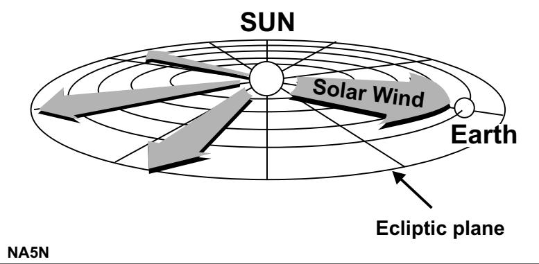
Fig. 12 – Classical model of the Sun's Electric Field and flow of the Solar Wind
